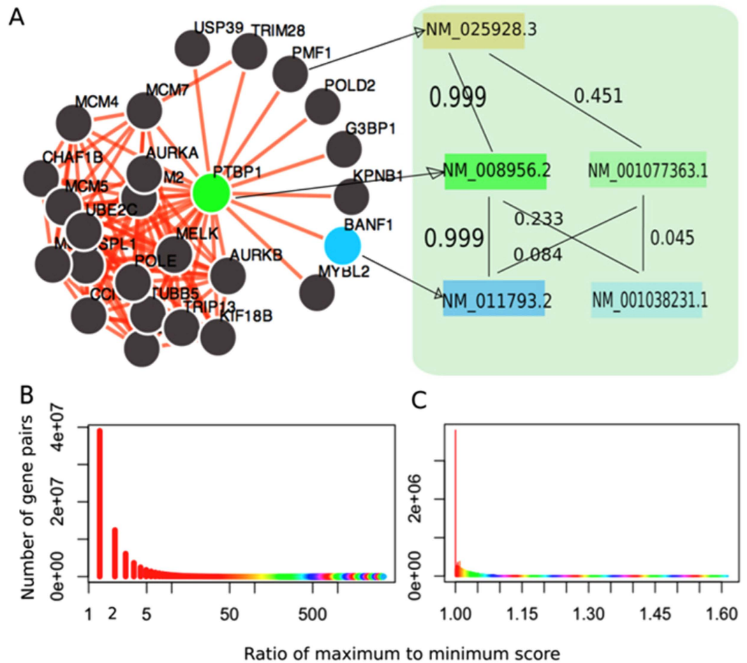
Figure 6. The isoform-level network reveals a high-resolution map of gene-gene co-functionality. (A) The left panel displays a traditional gene network of Ptbp1 . The link between Ptbp1 and Banf1 can be dissected into 4 isoform-level linkages. (B) For each multi-isoform gene pair, we calculated the ratio of the maximum to minimum probability among all its isoform pairs as a measure of functional linkage diversity of different isoform pairs from the same gene pair. Shown here is the distribution of this ratio of 75,512,782 gene pairs. 25% of the gene pairs have a value larger than 3. (C) We also calculated the ratios of maximum to minimum score of multi-isoform gene pairs using a random network built with shuffled gold standard. The values fall into a short range from 0 to 1.60, suggesting the significance of functional diversity of different isoform pairs of a gene pair.
