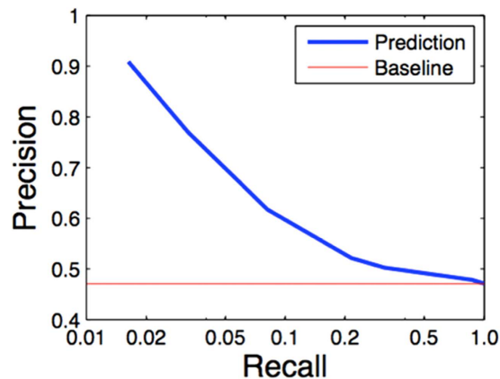
Figure 5. Experimental testing of the predictions using the validated isoform level protein-protein interaction data from Corominas, R. et al. Nat Commun, 2014 (Ref. 23).
